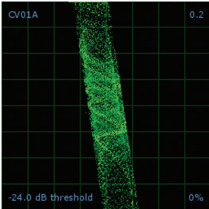
RIGHT CHANNEL IS INTERFERENCE - Right signal has been lost with a noisy loose connection and left channel crosstalk.
